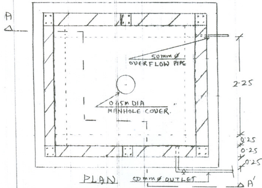
DETAILS OF OVERHEAD TANKS
